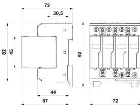
Dimension drawing
